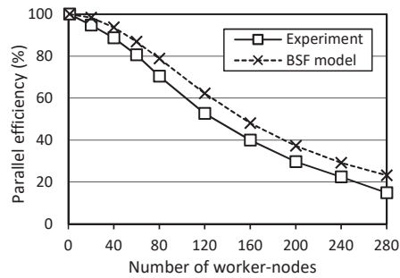
Figure 4. Experiments for n = 16000 and m = 32002
