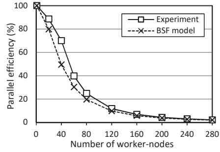
Figure 1. Experiments for n = 1500 and m = 3002
