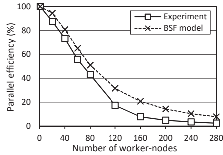
Figure 2. Experiments for n = 5000 and m = 10002
