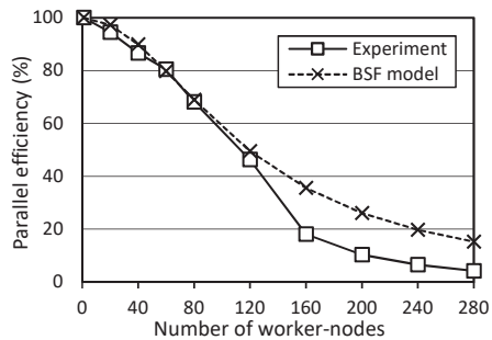
Figure 3. Experiments for n = 10000 and m = 20002
