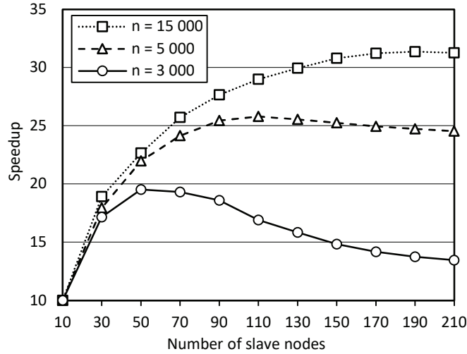
Fig. 2. Speedup curves of the FRaGenLP parallel algorithm for various dimensions
